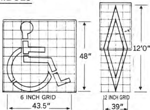
Handicapped parking symbol Diamond symbol H38" SYMBOL DL SYMBOL H48" SYMBOL
