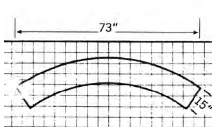
UCS SHAFT REVERSIBLE TURN BAY * SPECIFY FOR RIGHT OR LEFT MOVEMENT
