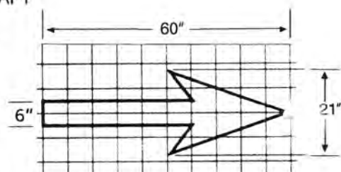
BIKE LANE ARROW
